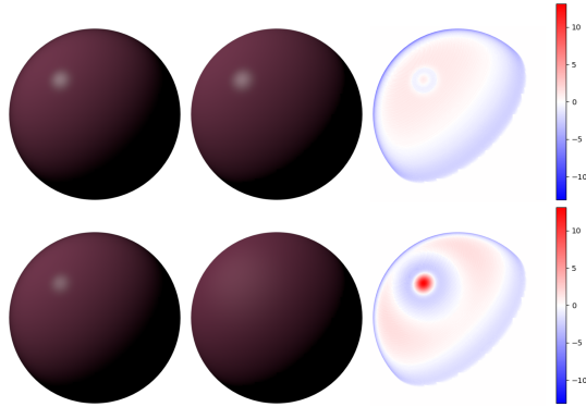
Figure 8: Source model (left), remapped target (center) and percentage error (right), corresponding to IOR = 1.3 (up) and IOR = 1.34 (down) in Figure 7.
