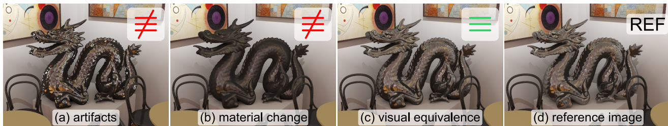
Figure 1: Examples of inequivalent and equivalent VPL rendering. (a)-(b) are VPL renderings with 1k VPLs, and clamp levels C1 = 316 and C8 = 0.1 , respectively, that are not equivalent ( \neq ) to the reference (d) because they have image artifacts (a) or different perceived material appearance (b). (c) VPL rendering produces an image that is visually equivalent ( \equiv ) to the reference for 100k VPLs and clamp level C4 = 10 , even though some reflections are lost where the Dragon is in contact with the pedestal and around its silhouette.
