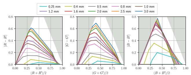
Fig. 11. Convex hulls of the achievable color pairs in the mean-difference representation for each channel and thickness of the object. Each convex hull represents around 4000 data points.
